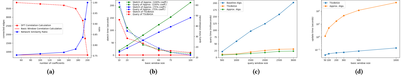
Figure 3: In-memory: (a) Network Accuracy Comparison (b) Basic Window Size Analysis (c) Query Window Size Analysis (d) Network Update Time.
