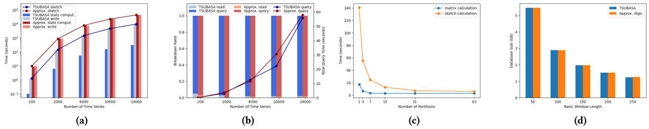
Figure 4: Parallel and Disk-based: (a) Sketch Time Breakdown (b) Query Time Breakdown (c) Impact of Parallelization (d) Space Overhead.
